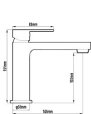
BRUNETTI BASIN MIXER CODE 69005, 69005B, 69005BC, 69005BG, 69005BR, 69005GM 69005RG, 69005W
