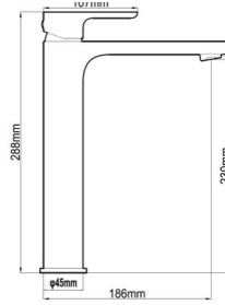
BASSINI BASIN MIXER EXT CODE 82805-T, 82805-T-B, 82805-T-BC, 82805-T-BG, 82805-T-BR, 82805-T-GM 82805-T-RG, 82805-T-W
