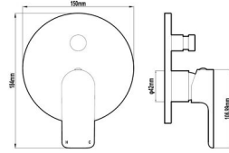
BASSINI WALL DIVERTER MIXER CODE 82811, 82811-B, 82811-BC, 82811-BG, 82811-BR, 82811-GM 82811-RG, 82811-W
