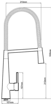
BASSINI SINK MIXER CODE 89001
